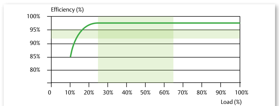
Liebert 80-eXL AC/AC efficiency with MSS Intelligent Paralleling feature.
