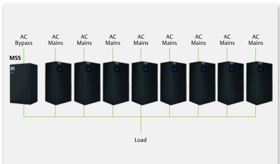
Liebert 80-eXL centralized parallel configuration, with MSS plus 8 UPS units in parallel.
