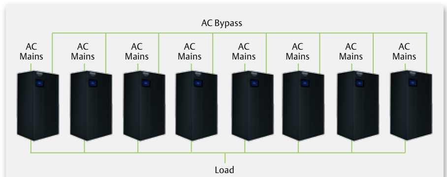
Liebert 80-eXL distributed parallel configuration, with 8 UPS units in parallel.
